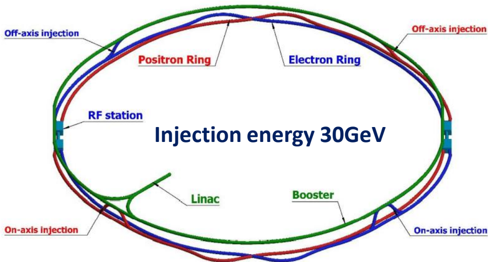
CEPC booster ring (100km)
