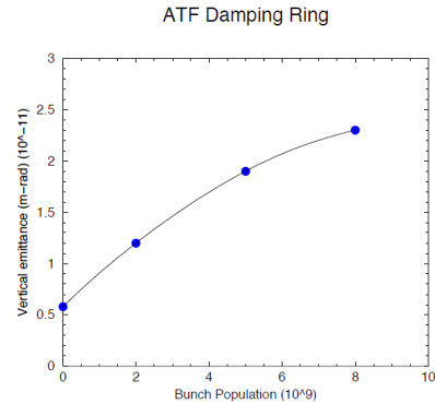
Figure 9.4: Vertical emittance vs bunch population. The dots and solid line correspond to the experimental and theoretical values, respectively.
