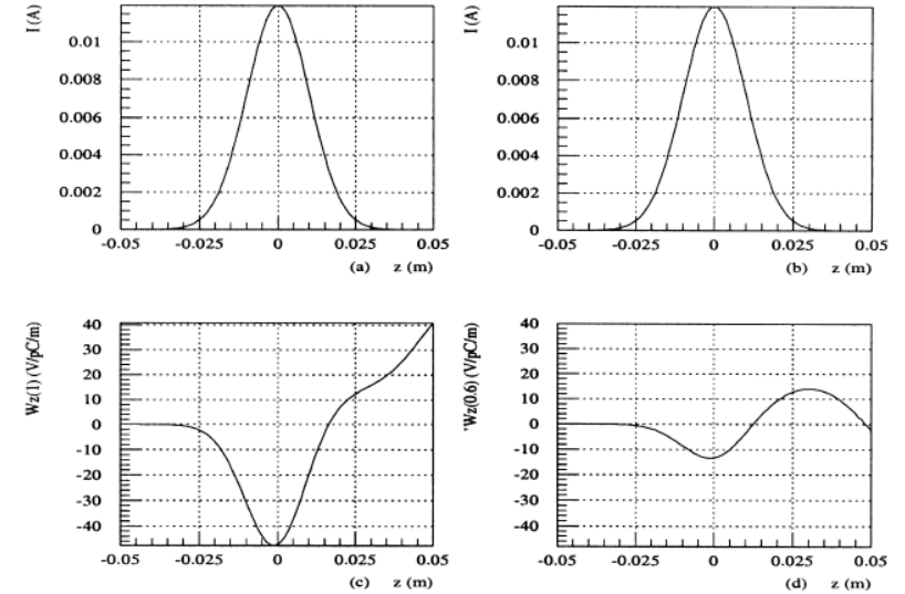
Fig. 5. A closed pill-box case: a = 0 , h = D = 0.035 m and \sigma_z = 0.01 m. (a) and (b) are the Gaussian bunch current distributions of the point charge and (c) and (d) are the longitudinal wakefields at (c) \beta = 1 , and (d) \beta = 0.6 .
